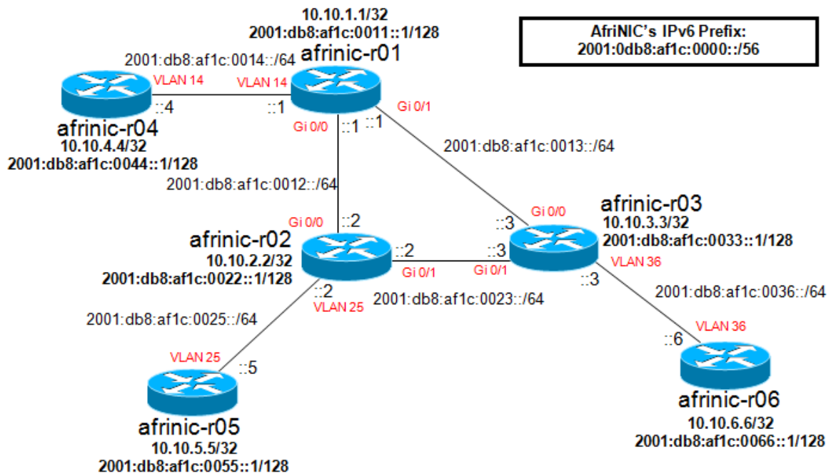
Esquema Testbed AfriNIC
